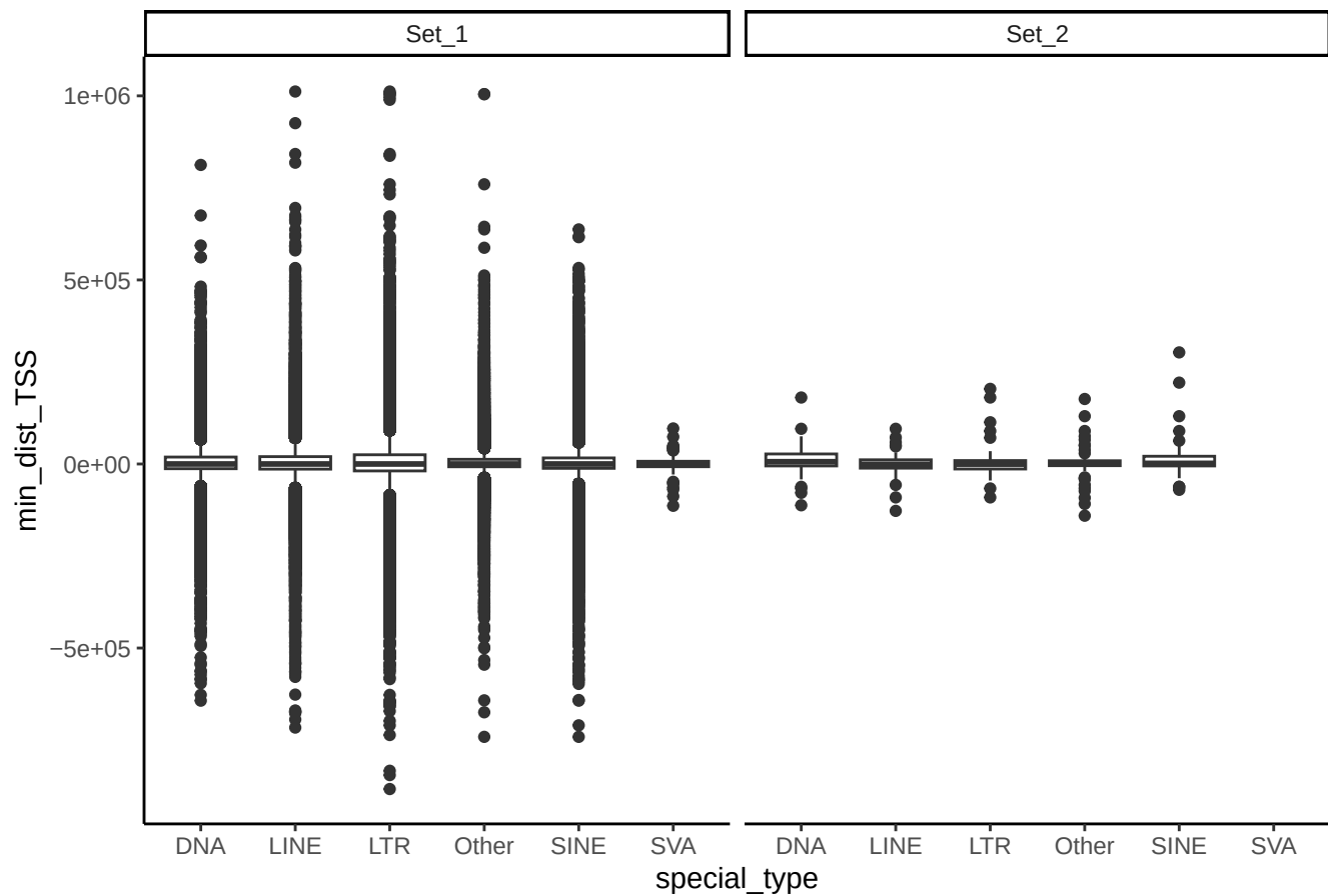
Distance to TSS per class in H3K27me3 of overlapping ROIs
